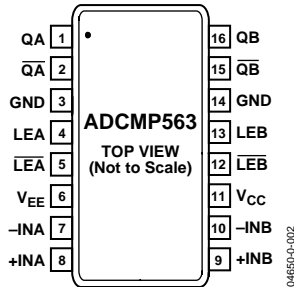
Figure 4. ADCMP563 16-Lead QSOP Pin Configuration
