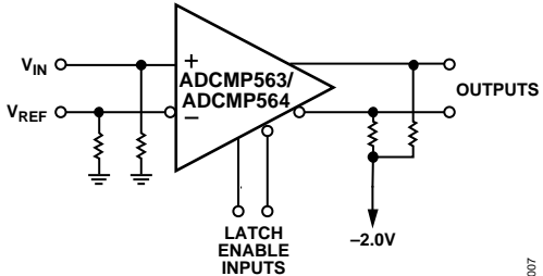
Figure 22. High Speed Sampling Circuits
