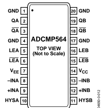
Figure 3. ADCMP564 20-Lead QSOP
