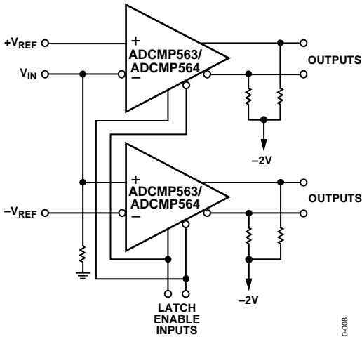
Figure 23. High Speed Window Comparator
