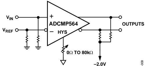
Figure 24. Adding Hysteresis Using the HYS Control Pin
